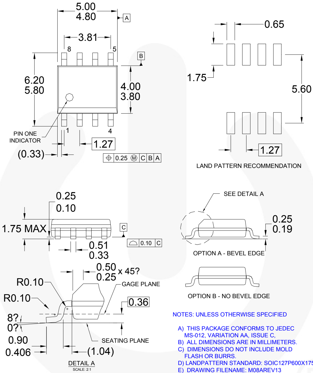
Figure 56. 8-Lead SOIC
