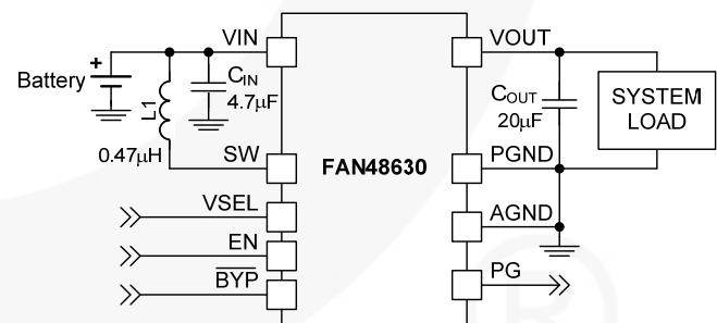
Figure 1. Typical Application
