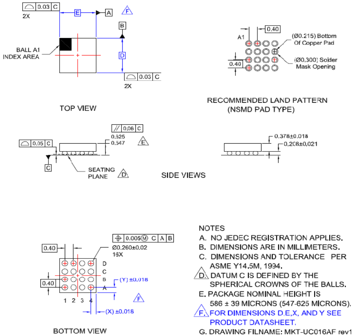
Figure 30. 16-Ball, 4x4 Array, 0.4 mm Pitch, 250 µm Ball, Wafer-Level Chip-Scale Package (WLCSP)
