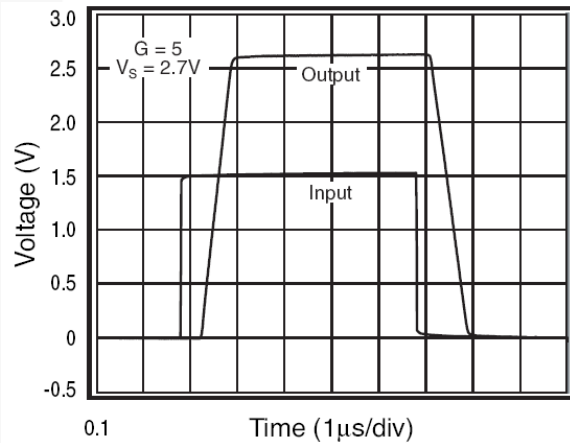
Figure 22. Overdrive Recovery
