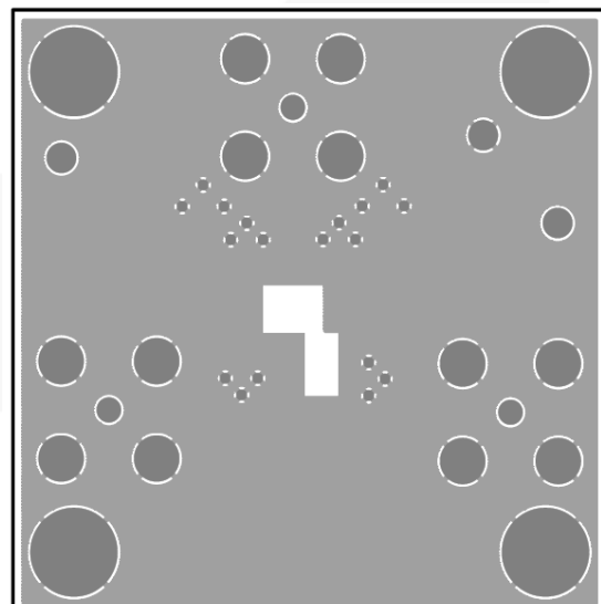
Figure 26. Bottom Side
