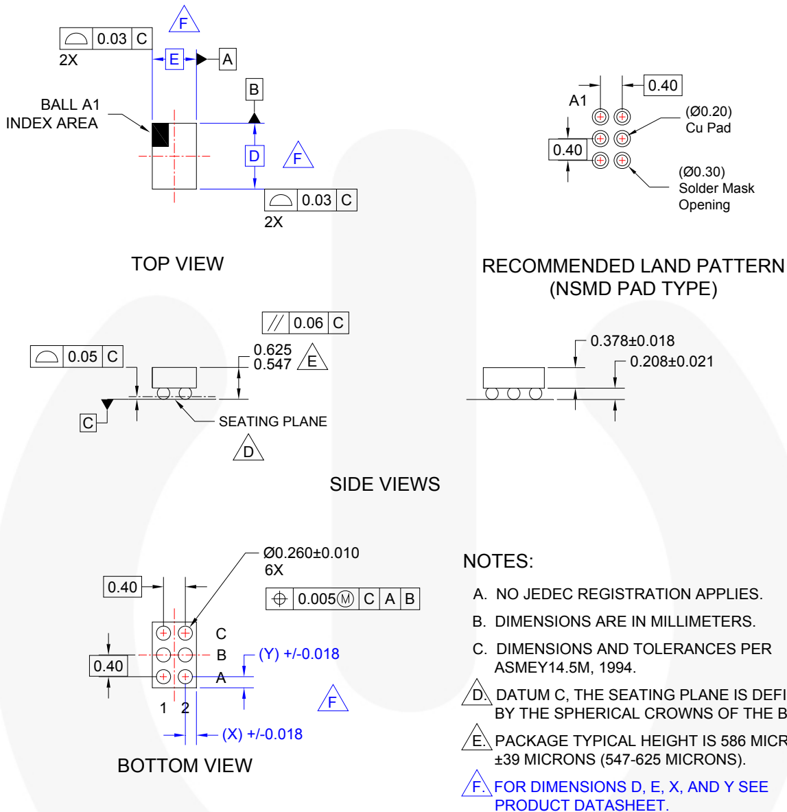
Figure 1. 6-Bump WLCSP, 0.4mm Pitch
