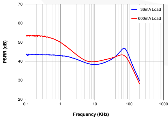
Figure 30. PSRR, 50 \Omega and 3 \Omega Load
