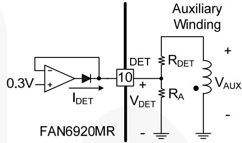
Figure 41. Valley Detection
