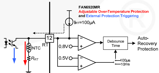
Figure 45. Adjustable Over-Temperature Protection
