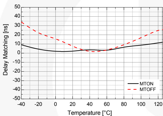
Figure 12. Delay Matching vs. Temperature
