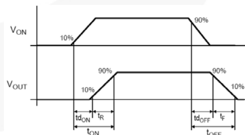
Figure 27. Timing Diagram
