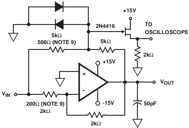
FIGURE 1. LARGE SIGNAL RESPONSE CIRCUIT
