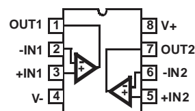
HA-5104 (PDIP, Cerdip) TOP VIEW
