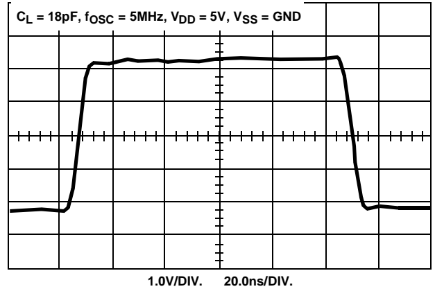
FIGURE 6. OUTPUT WAVEFORM ( C_L = 18\text{pF} )
