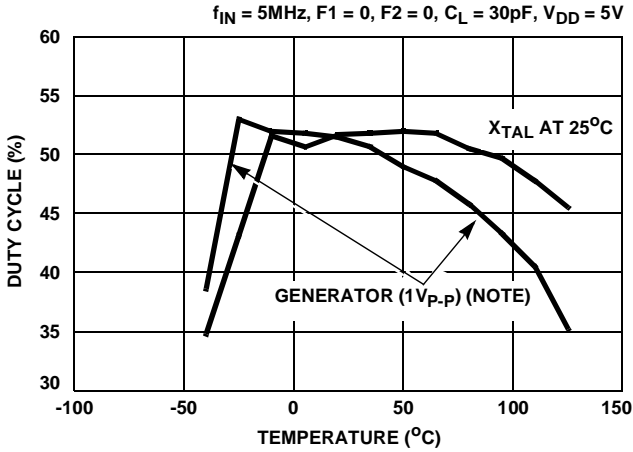
FIGURE 23. DUTY CYCLE vs TEMPERATURE
