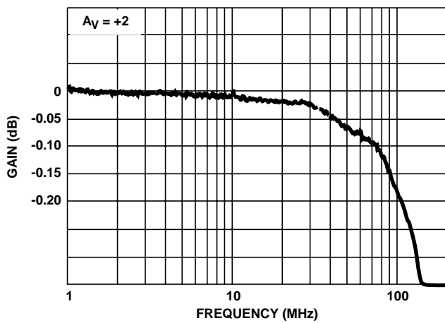
FIGURE 15. GAIN FLATNESS
