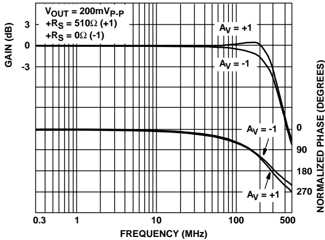
FIGURE 13. FREQUENCY RESPONSE
