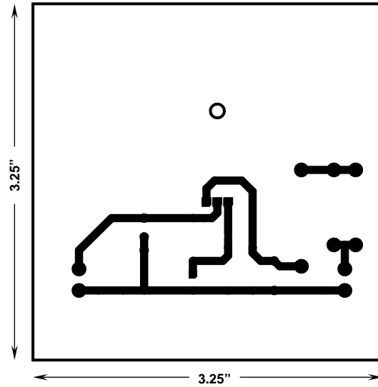
FIGURE 2. EVALUATION BOARD METAL MASK (BOTTOM)
