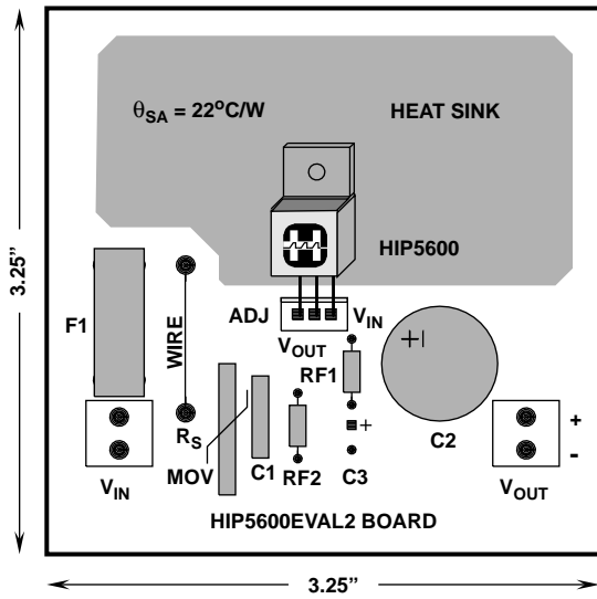
FIGURE 1. EVALUATION BOARD (TOP)
