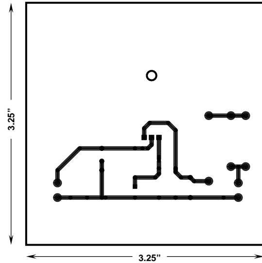
FIGURE 2. EVALUATION BOARD METAL MASK (BOTTOM)
