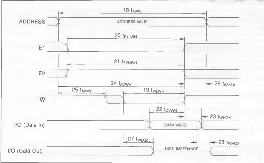
Figure 2.4 WRITE CYCLE 1
