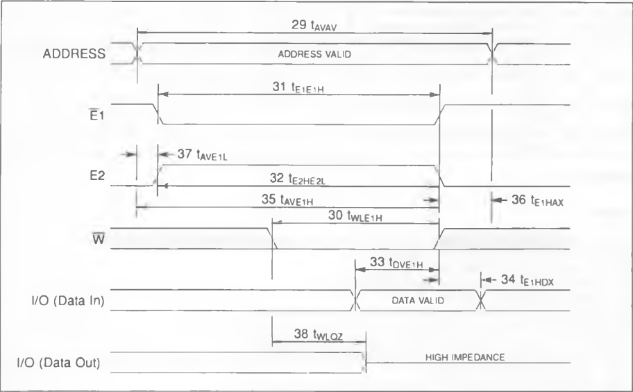
Figure 2.5 WRITE CYCLE 2
