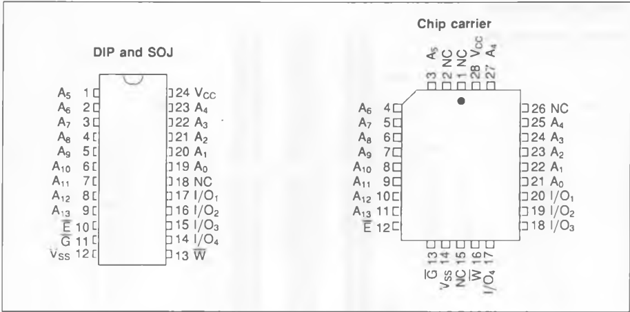
Figure 2.10 16K x 4 (with output enable) pin configuration
