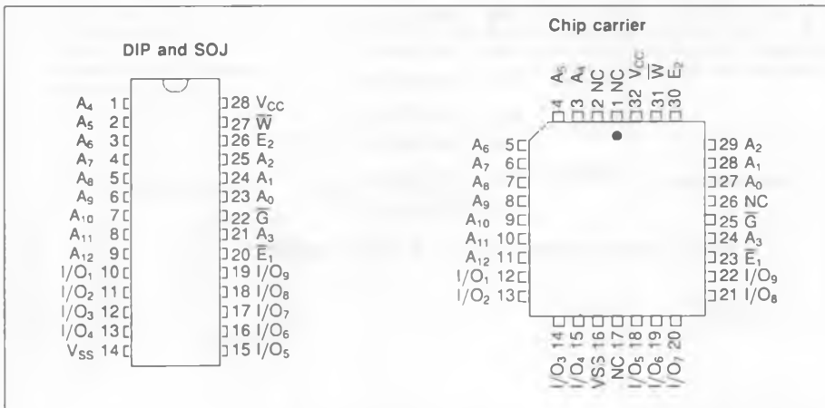
Figure 2.13 8K x 9 pin configuration
