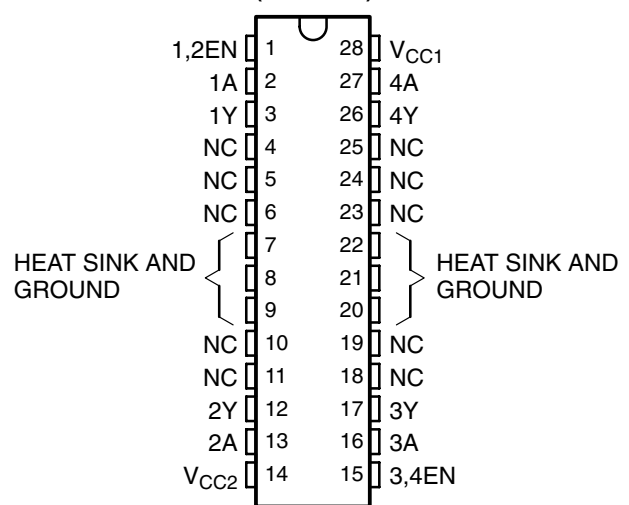
L293 . . . DWP PACKAGE (TOP VIEW)
