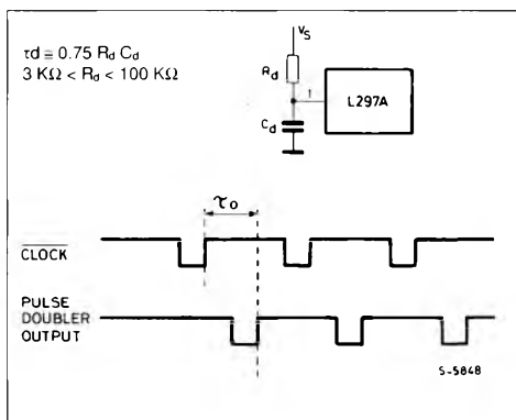
Figure 4 : Pulse doubler (L297A)
