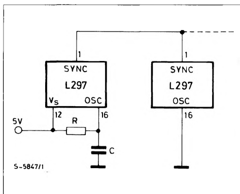
Figure 3 : Synchronising L297s
