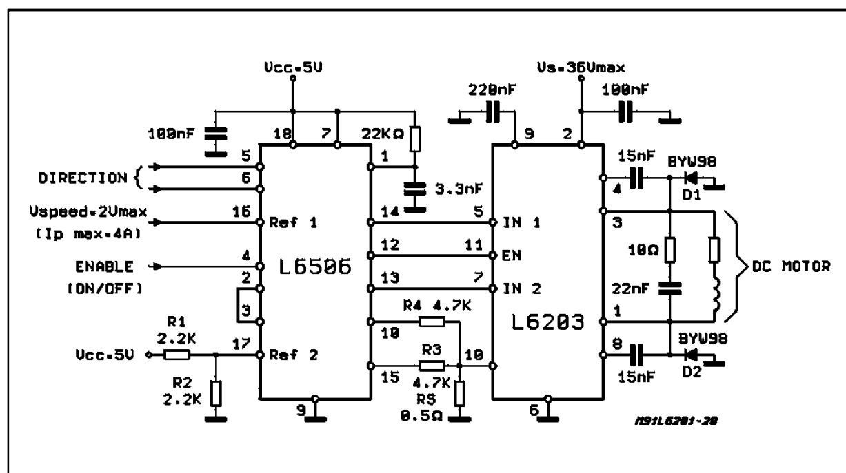
Figure 17: Bidirectional DC Motor Control
