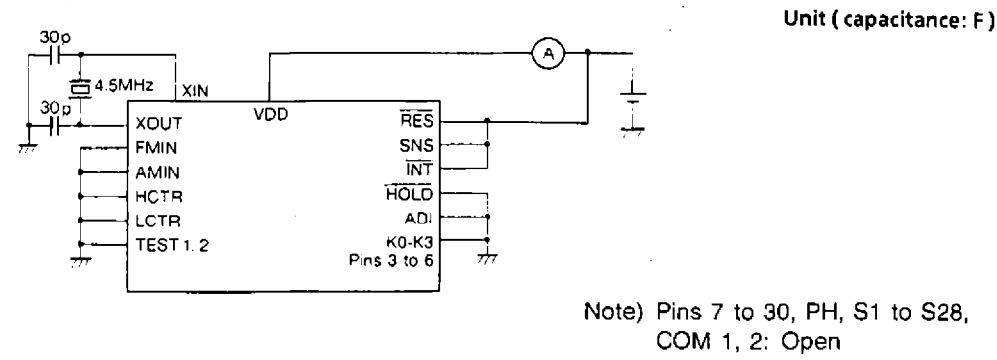
Fig. 1 I DD (2) at HOLD Mode
