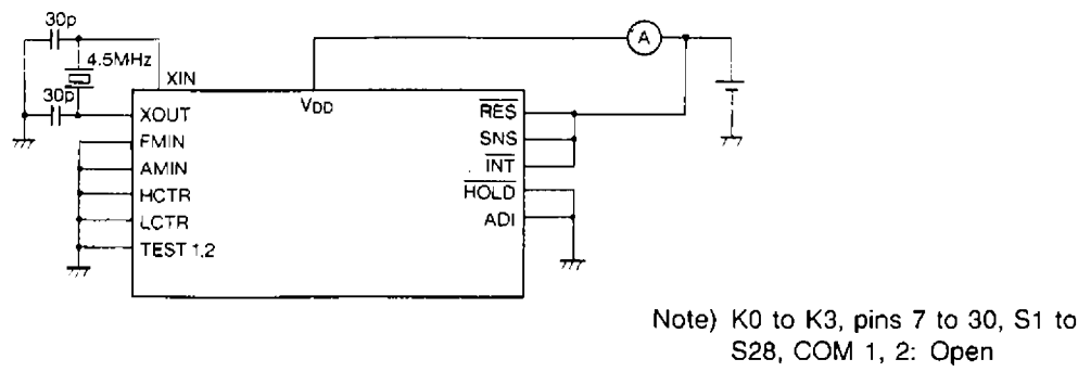
Fig. 2 I DD (3) at Backup Mode
