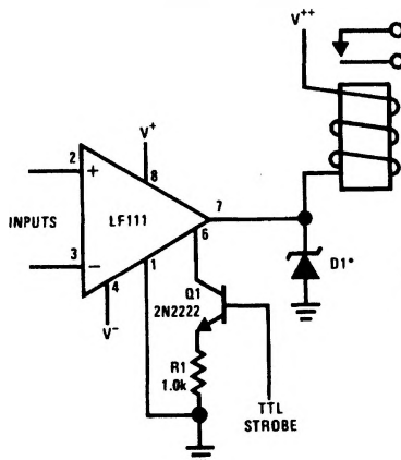
Relay Driver with Strobe
