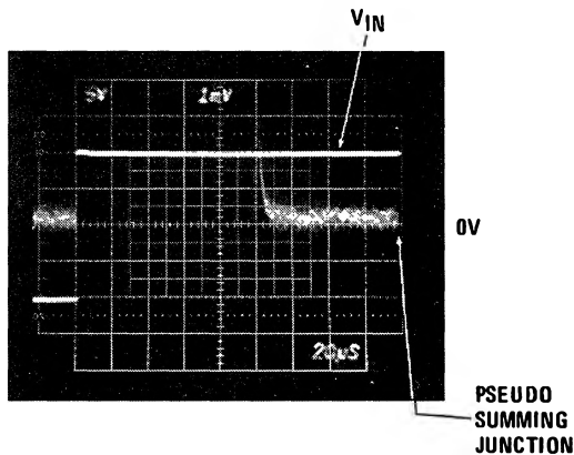
FIGURE 12. Settling Time
