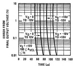
FIGURE 14. Settling Time
