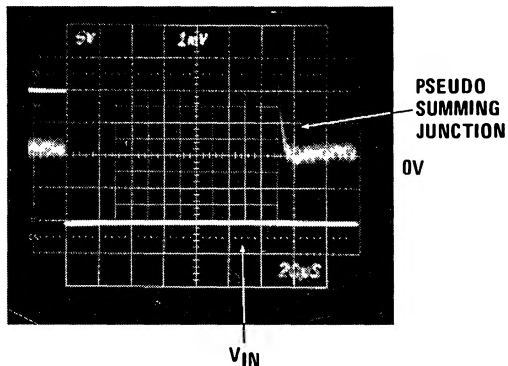
FIGURE 11. Settling Time
