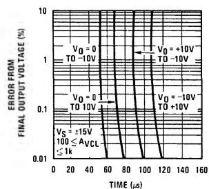
FIGURE 14. Settling Time
