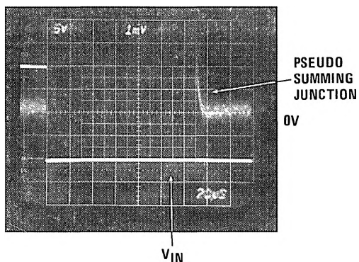
FIGURE 11. Settling Time
