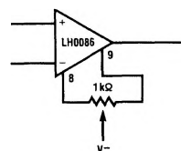
FIGURE 5. Offset Adjustment
