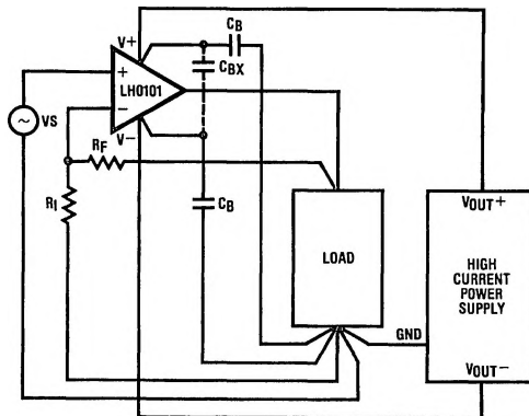
FIGURE 1. Single-Point Grounding
