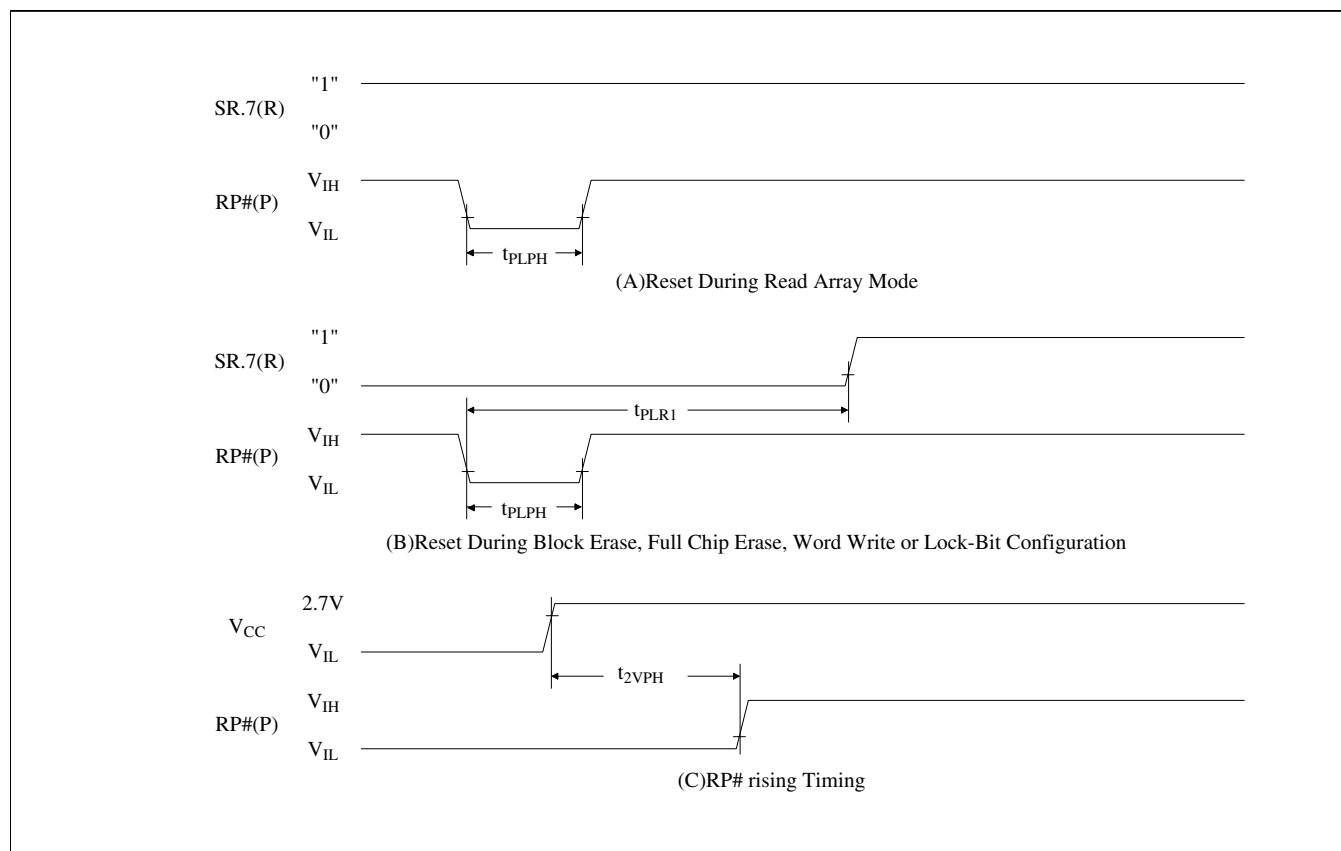
Figure 17. AC Waveform for Reset Operation
