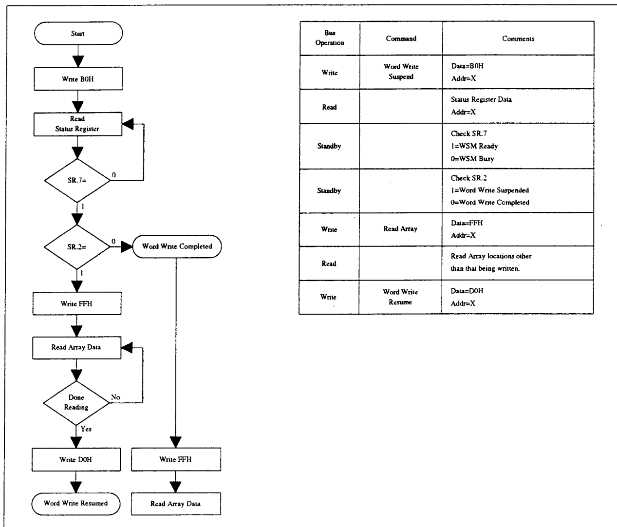
Figure 9. Word Write Suspend/Resume Flowchart
