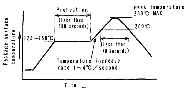
Recommended Reflow Soldering(Air) Temperature Profile
