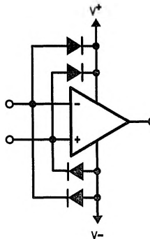
FIGURE 1. Clamping Inputs of Op Amp
