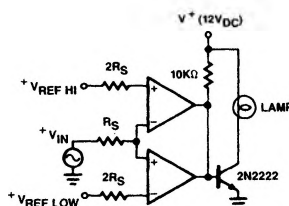
Limit Comparator
