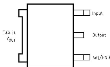
Figure 4. TO-263 Top View
