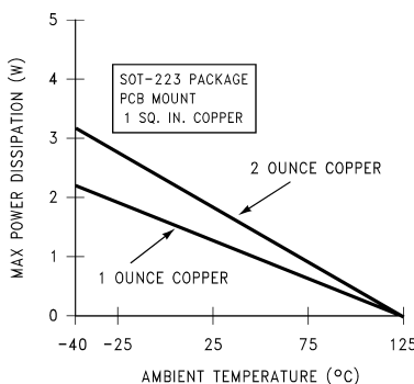
Figure 15. Maximum Power Dissipation vs T_{AMB} for the SOT-223 Package
