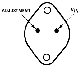
Figure 3. TO-3 (K) Metal Can Package
