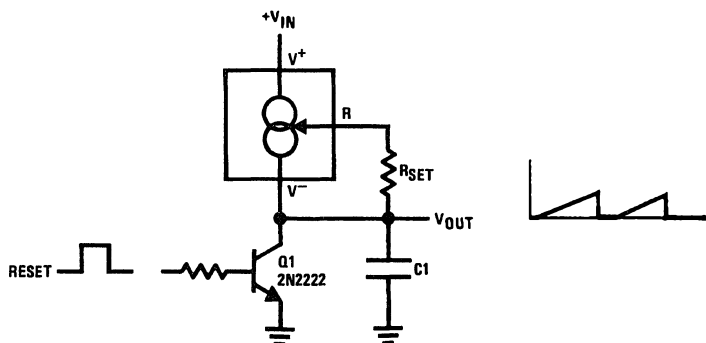
Ramp Generator
