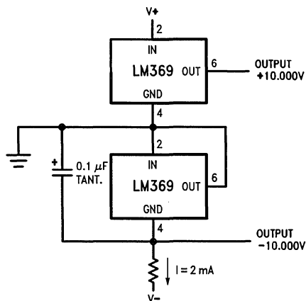
±10V Reference
