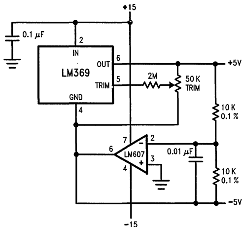
±5V Reference
