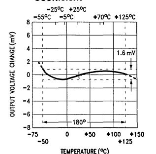
LM169 Temperature Coefficient
