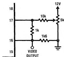
FIGURE 2. Adjustable Recovered Video Level
