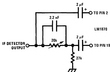
IF Correction Lead Network
