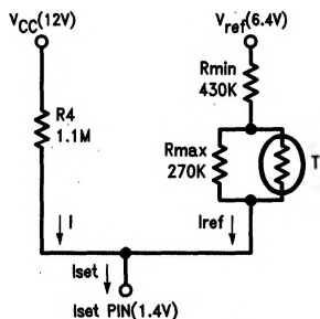
FIGURE 8. Thermistor/Resistor Network
