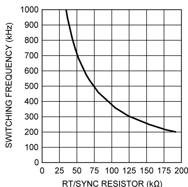
Figure 18. Switching Frequency vs RT/SYNC Resistor
