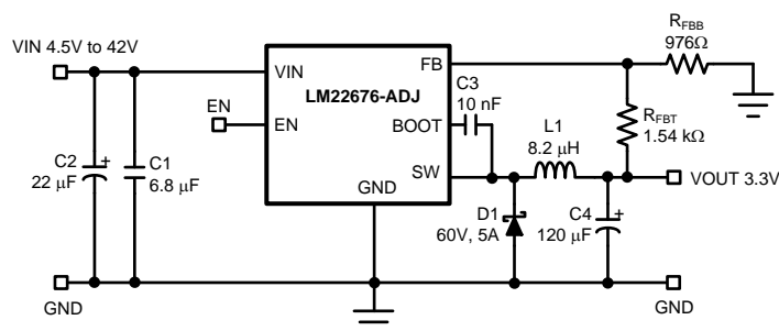
Figure 16. Typical Buck Regulator Application
