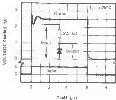
RESPONSE TIME
