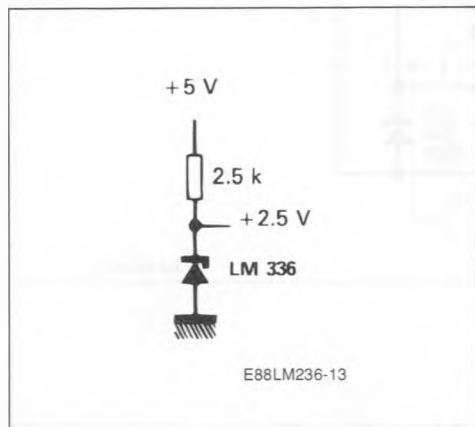
Figure 3 : 2.5 V Reference.
