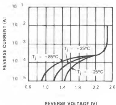
REVERSE CHARACTERISTICS
