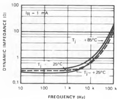
DYNAMIC IMPEDANCE
