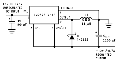
FIGURE 10. Inverting Buck-Boost Develops -12V
