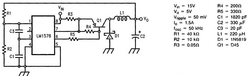
FIGURE 4. Buck Converter with Boosted Output Current
