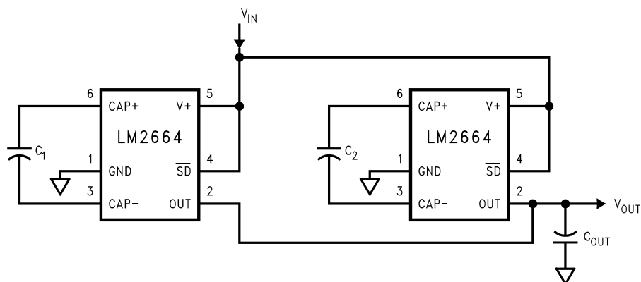
Figure 16. Lowering Output Resistance by Paralleling Devices
