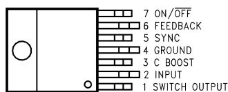
Figure 2. TO-220 Package Top View
