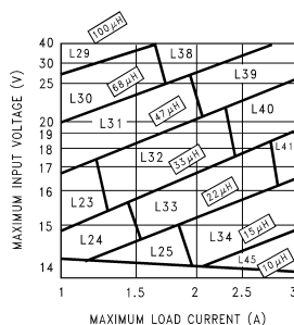
Figure 12. LM2670-12EP
