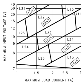
Figure 11. LM2670-5.0EP
