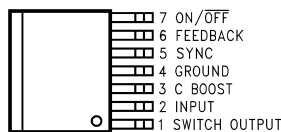
Figure 1. TO-263 Package Top View
