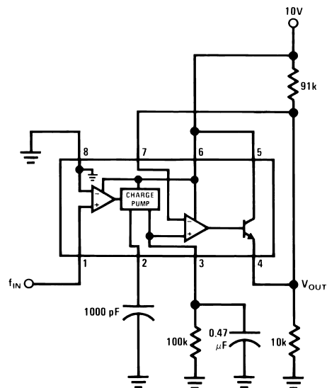
Figure 21. Changing Tachometer Gain Curve or Clamping the Minimum Output Voltage
