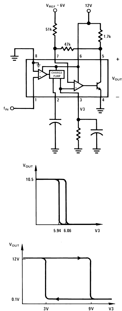
Figure 20. Changing the Output Voltage for an Input Frequency of Zero
