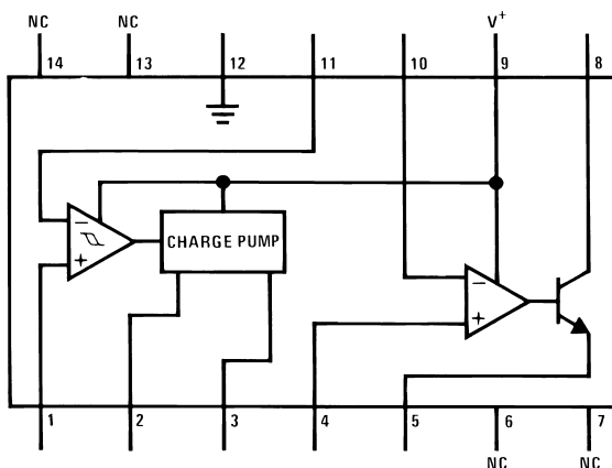
Figure 3. LM2907
