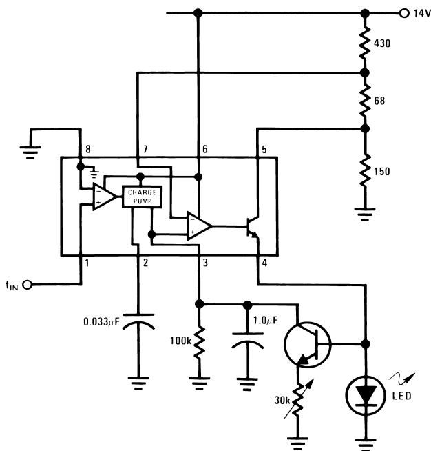
Figure 16. Flashing LED Indicates Overspeed
