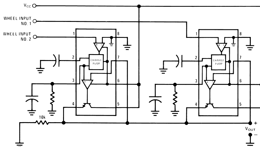
Figure 23. “Select-High” Circuit
