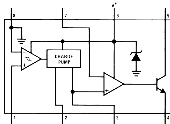
Figure 2. LM2917-8
