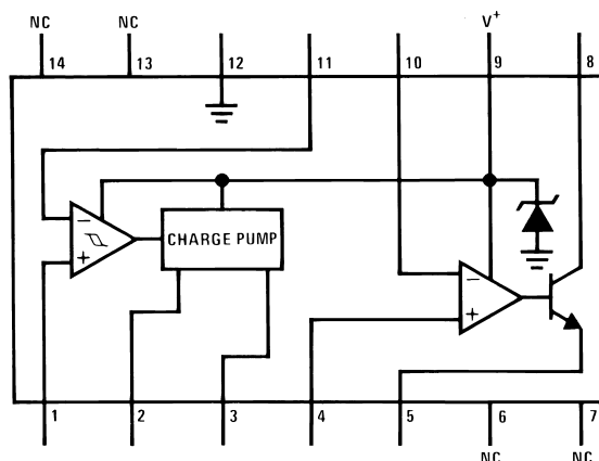
Figure 4. LM2917
