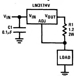
1A Current Regulator
