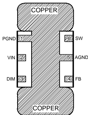
Figure 20. PCB Dog Bone Layout
