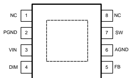
Figure 3. 8-Pin MSOP-PowerPad (Top View) See GDN0008A Package
