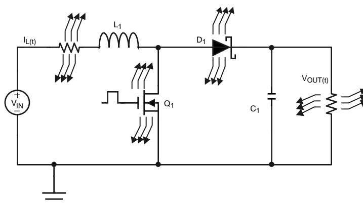
Figure 21. Thermal Schematic
