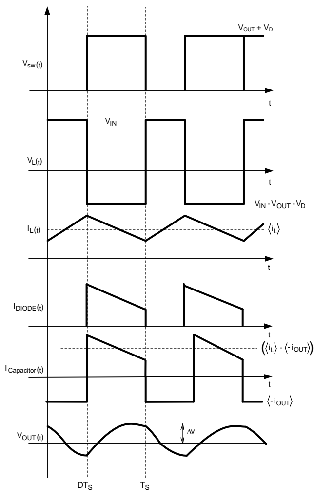
Figure 15. Typical Waveforms
