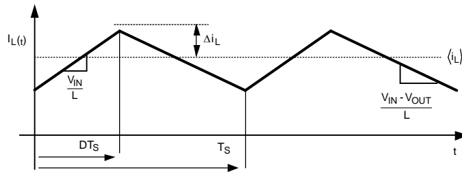
Figure 17. Inductor Current
