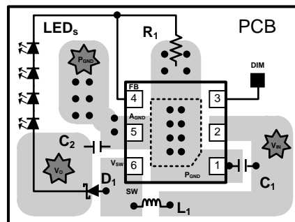
Figure 19. Boost PCB Layout Guidelines
