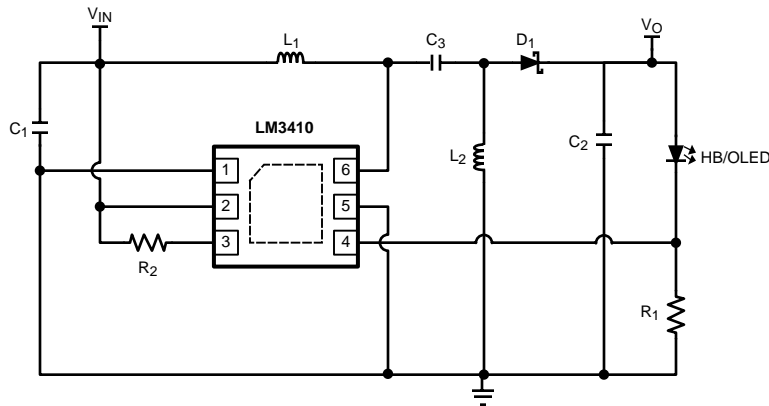
Figure 26. HB/OLED SEPIC CONVERTER Schematic
