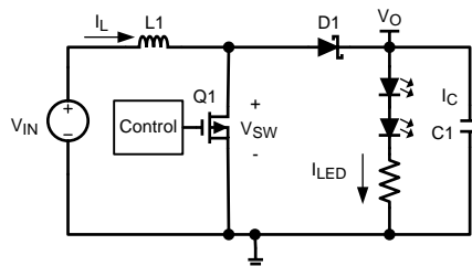
Figure 14. Simplified Boost Topology Schematic
