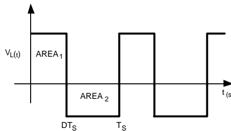
Figure 25. Inductor Volt-Sec Balance Waveform
