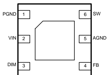
Figure 2. 6-Pin WSON (Top View) See NGG0006A Package
