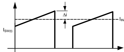
Figure 23. LM3410 Switch Current
