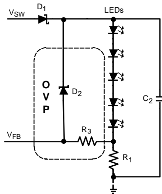
Figure 18. Overvoltage Protection Circuit
