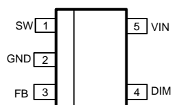
Figure 1. 5-Pin SOT-23 (Top View) See DBV Package
