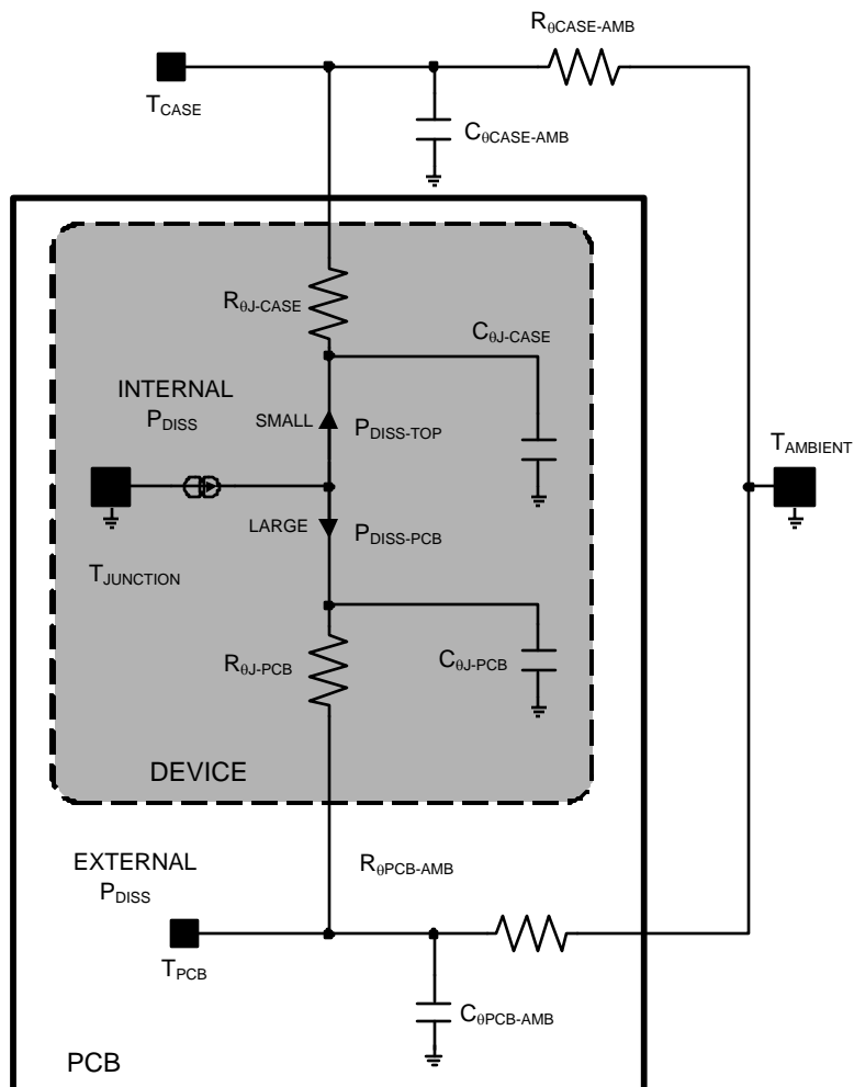
Figure 22. Associated Thermal Model
