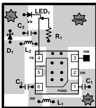
Figure 28. HB/OLED SEPIC PCB Layout
