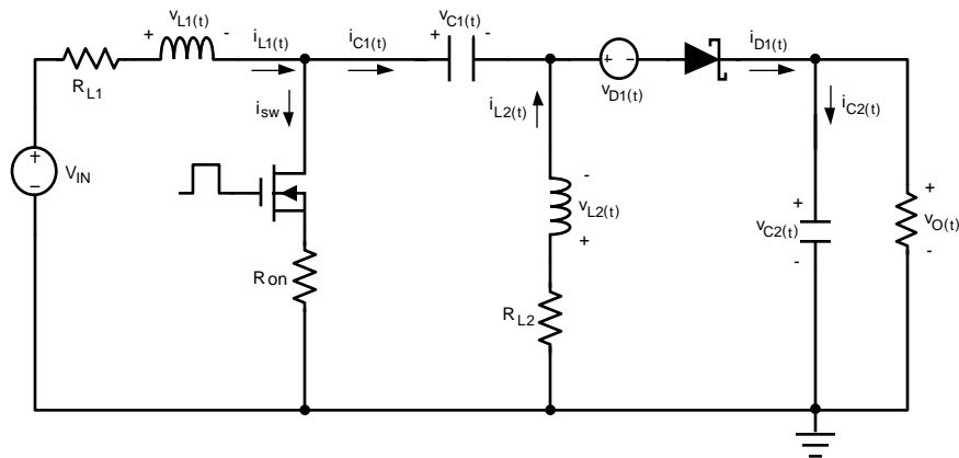
Figure 27. SEPIC Simplified Schematic
