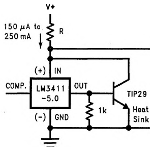
FIGURE 14. 250 mA Shunt Regulator
