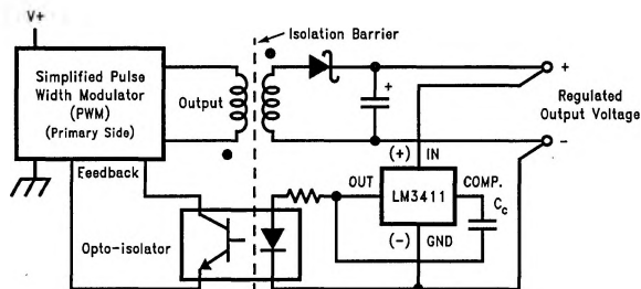
Basic Isolated DC/DC Converter
