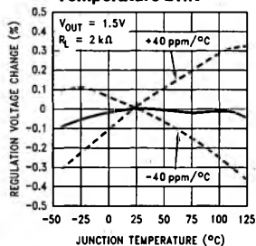
Normalized Temperature Drift
