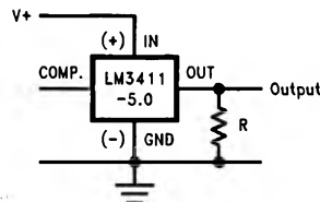
FIGURE 15. Voltage Detector
