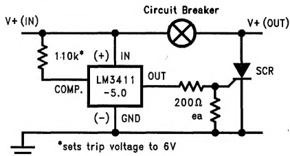
FIGURE 16. Overvoltage Crowbar
