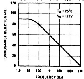
Common-Mode Rejection
