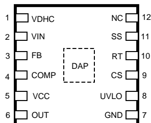
Figure 1. 12-Lead WSON Package
