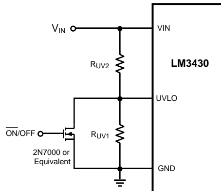
Figure 13. Enable/Disable Using UVLO
