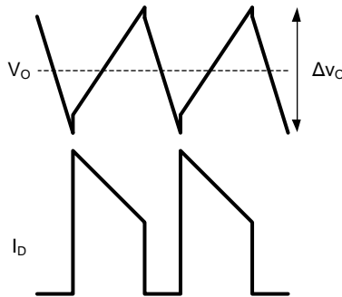
Figure 17. \Delta V_O Using Low ESR Capacitors
