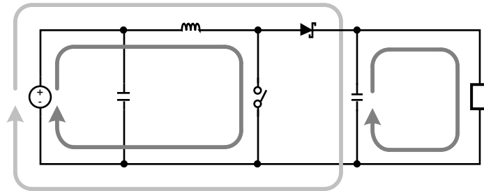
Figure 22. Boost Converter Current Loops
