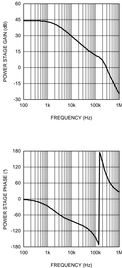
Figure 19. Power Stage Gain and Phase
