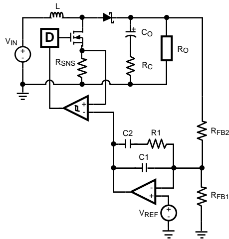
Figure 18. Power Stage and Error Amp
