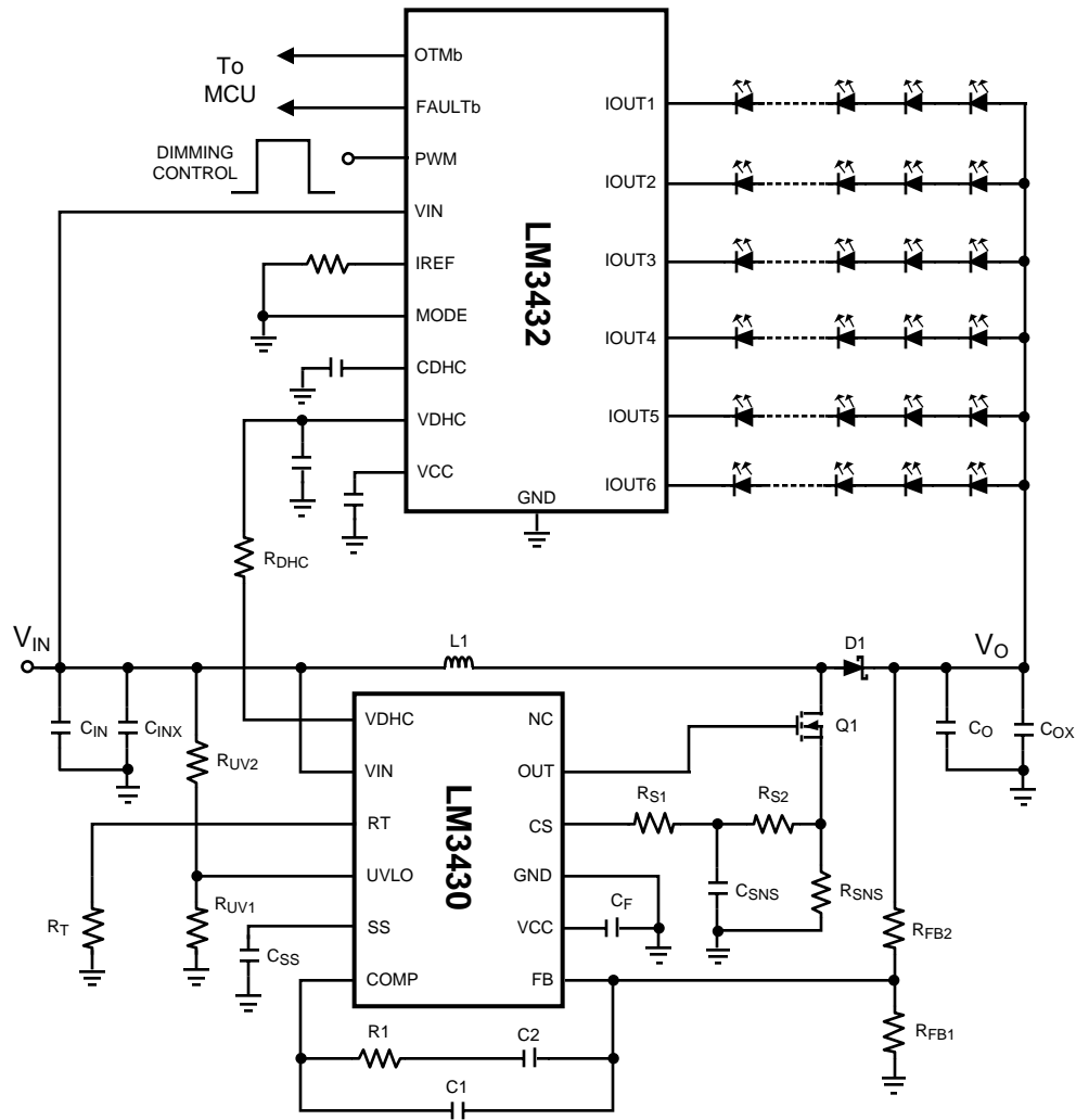
Figure 12. LM3430 with LM3432
