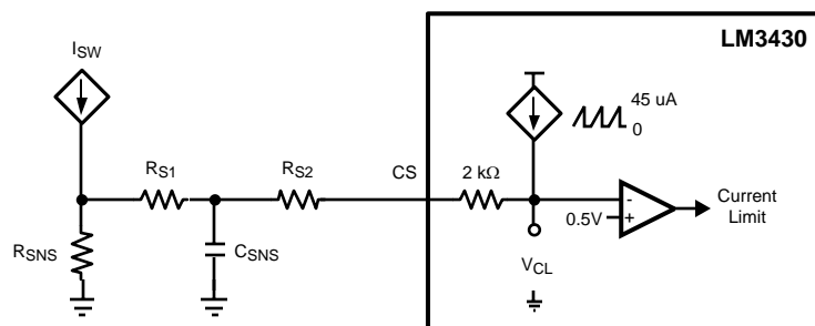
Figure 15. Slope Compensation
