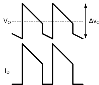
Figure 16. \Delta V_O Using High ESR Capacitors
