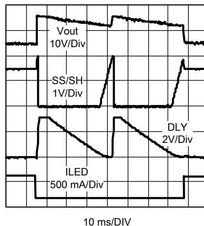
Figure 25. OVP and Auto-Restart
