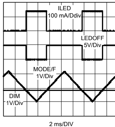
Figure 22. Analog Dimming Mode Waveforms
