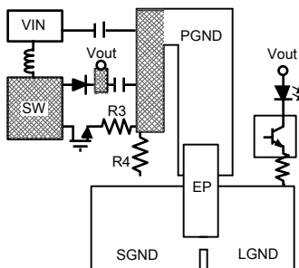
Figure 28. Example PCB Layout
