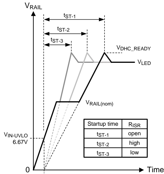
Figure 25. Setting different startup time using different R ISR
