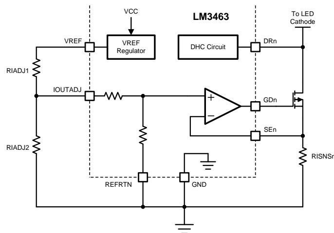
Figure 18. Block diagram of a linear current regulator
