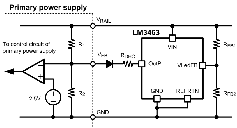
Figure 27. Connecting the LM3463 to a power supply
