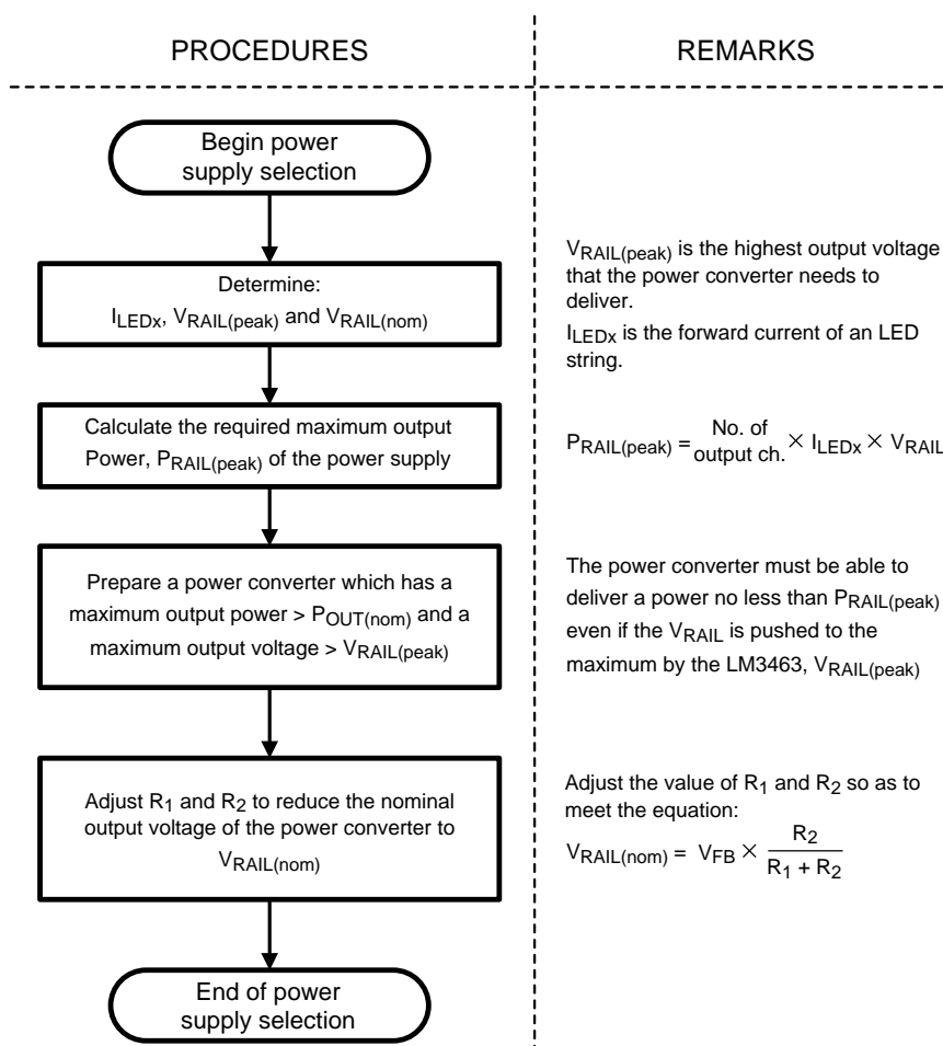
Figure 28. Procedures of selecting the primary power supply
