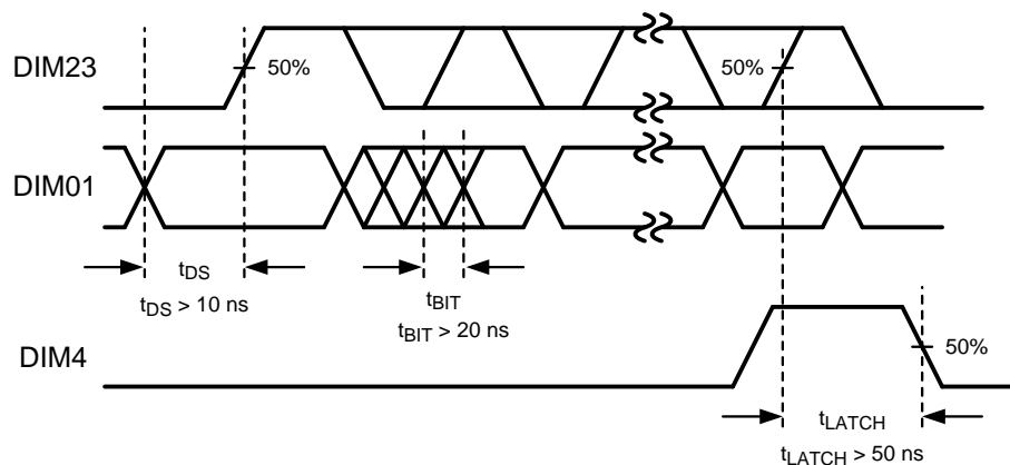
Figure 32. Timing parameters of the serial data interface
