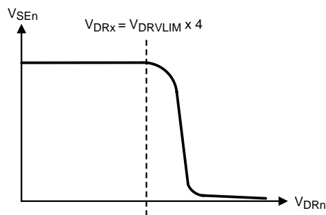
Figure 29. V_{\text{SEn}} reduces as V_{\text{DRn}} exceeds V_{\text{DRVLM}} \times 4
