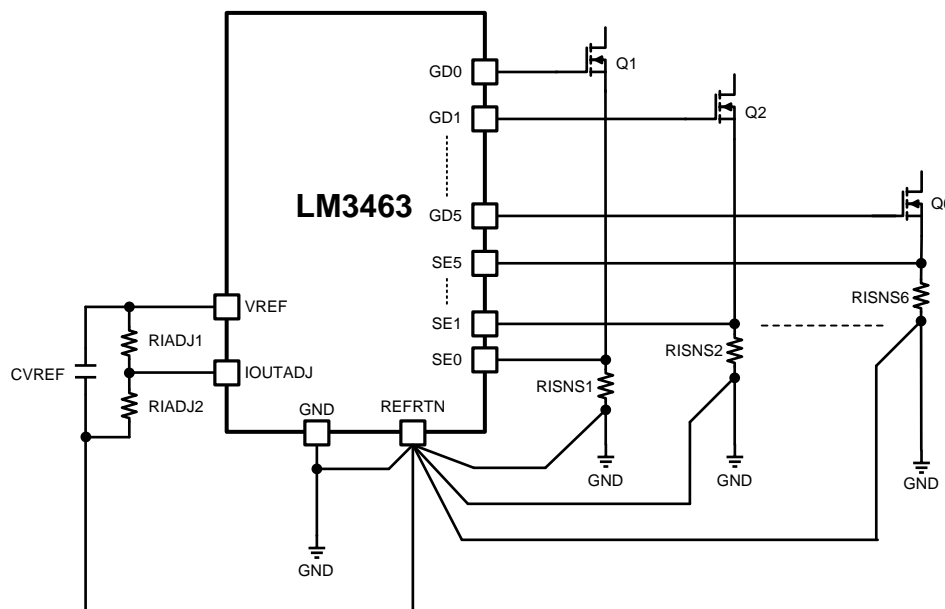
Figure 22. Individual connections to REFRTN
