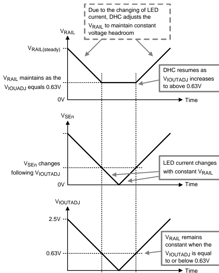
Figure 23. Holding V_{RAIL} when V_{IOUTADJ} is below 0.63V
