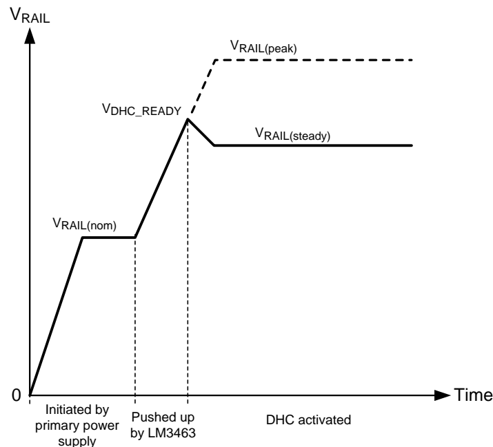
Figure 24. Changes of V_{RAIL} during system startup
