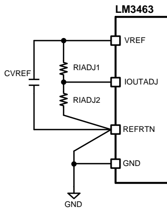
Figure 21. Biasing IOUTADJ from VREF
