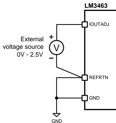
Figure 20. Adjust V_{SEn} by external voltage
