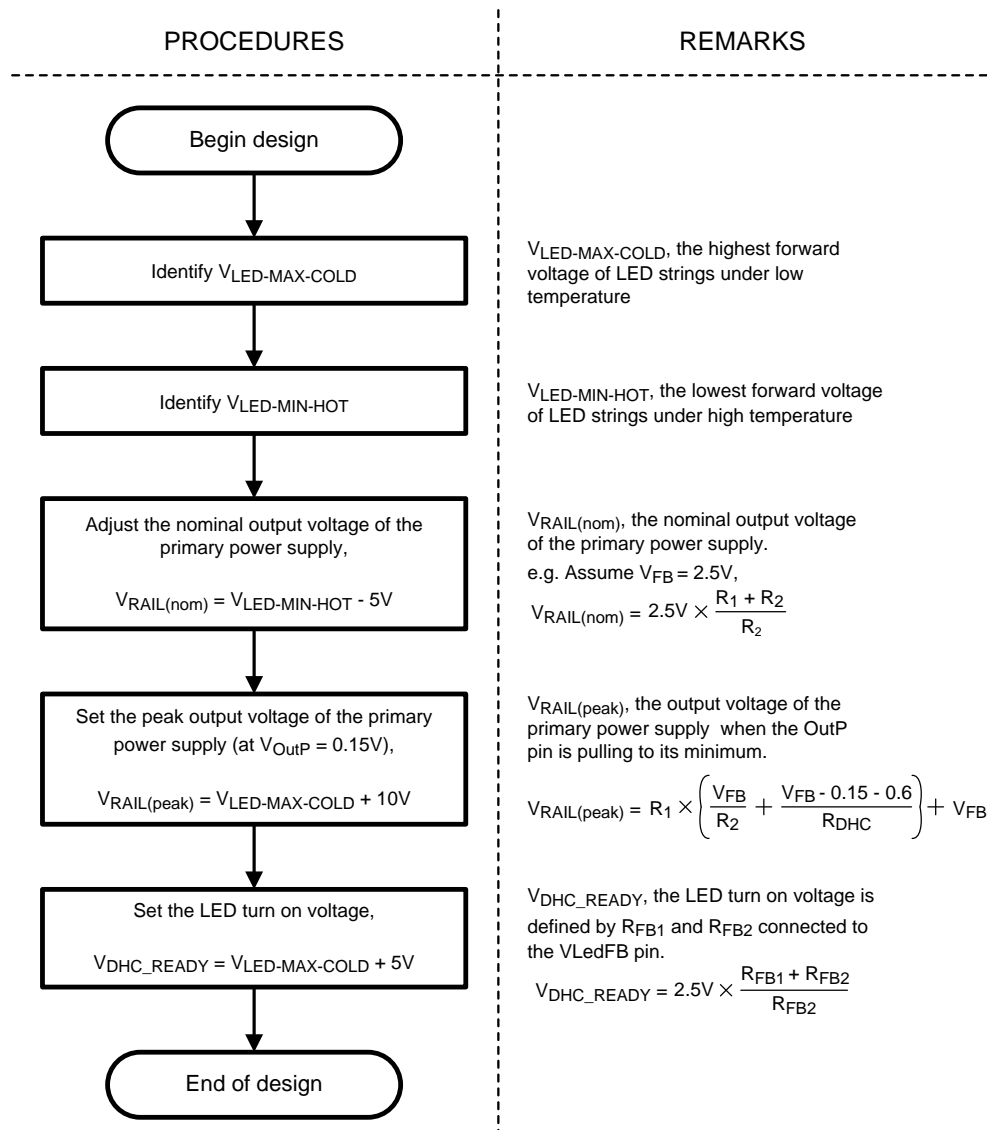
Figure 26. Procedure of defining startup parameters
